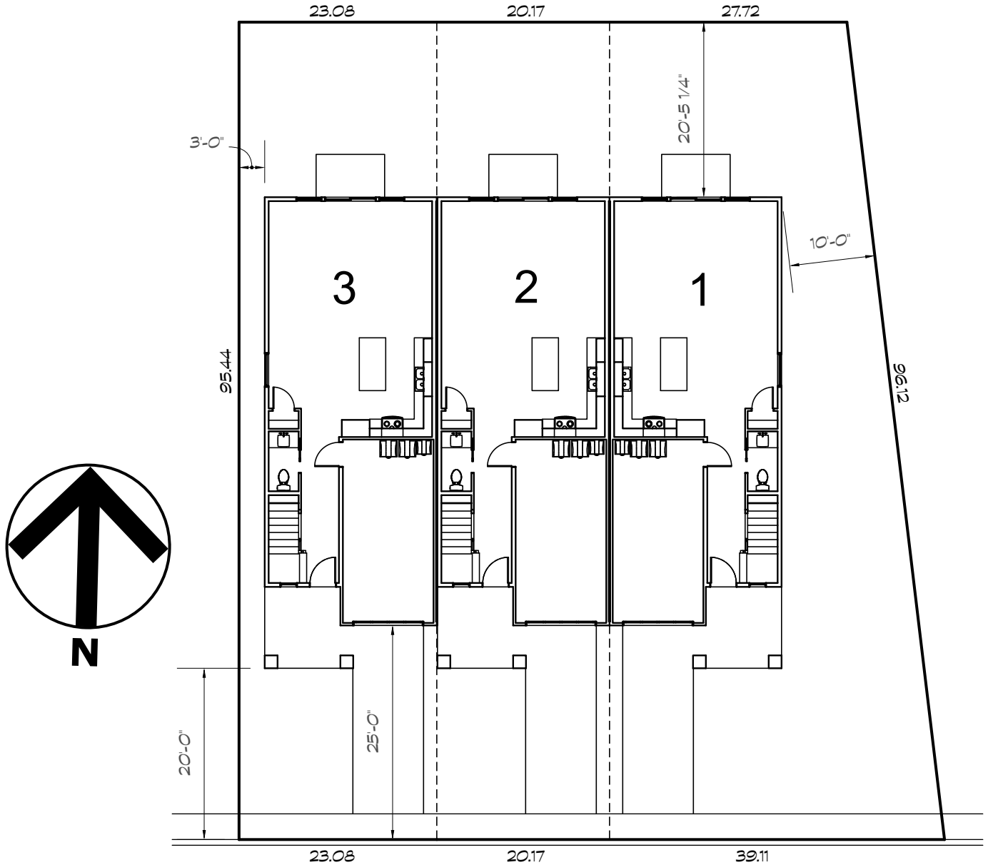
1 Site Plan scale 1/16"=1'-0"
